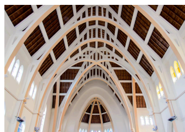
Charpente. Phot. Jean-Marc Ramette IVR32_20216205004NUCA
