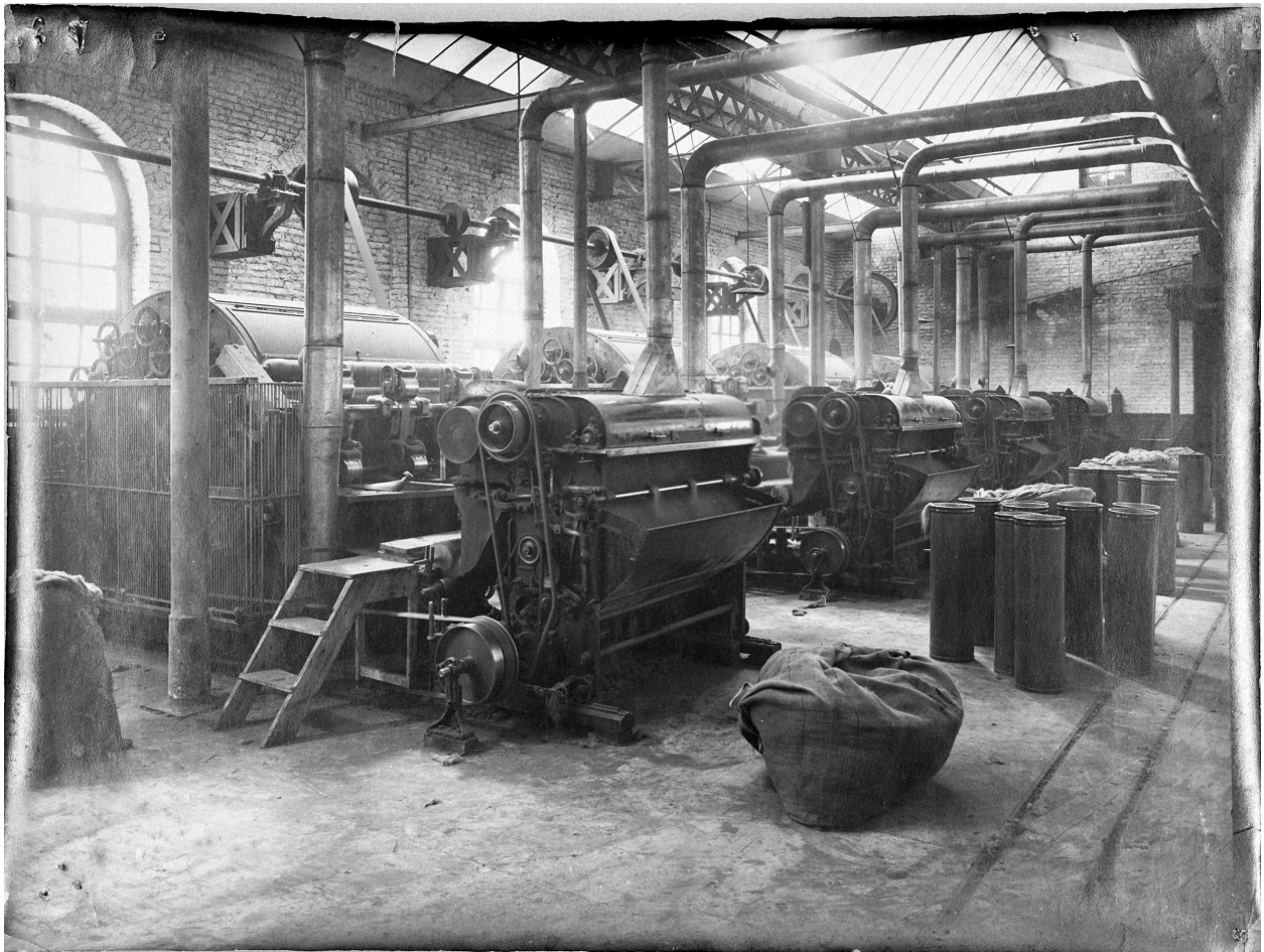
Ancienne filature. Cardeuses. Photographie, photographe inconnu, [circa 1900] (coll. part. Charvet).
