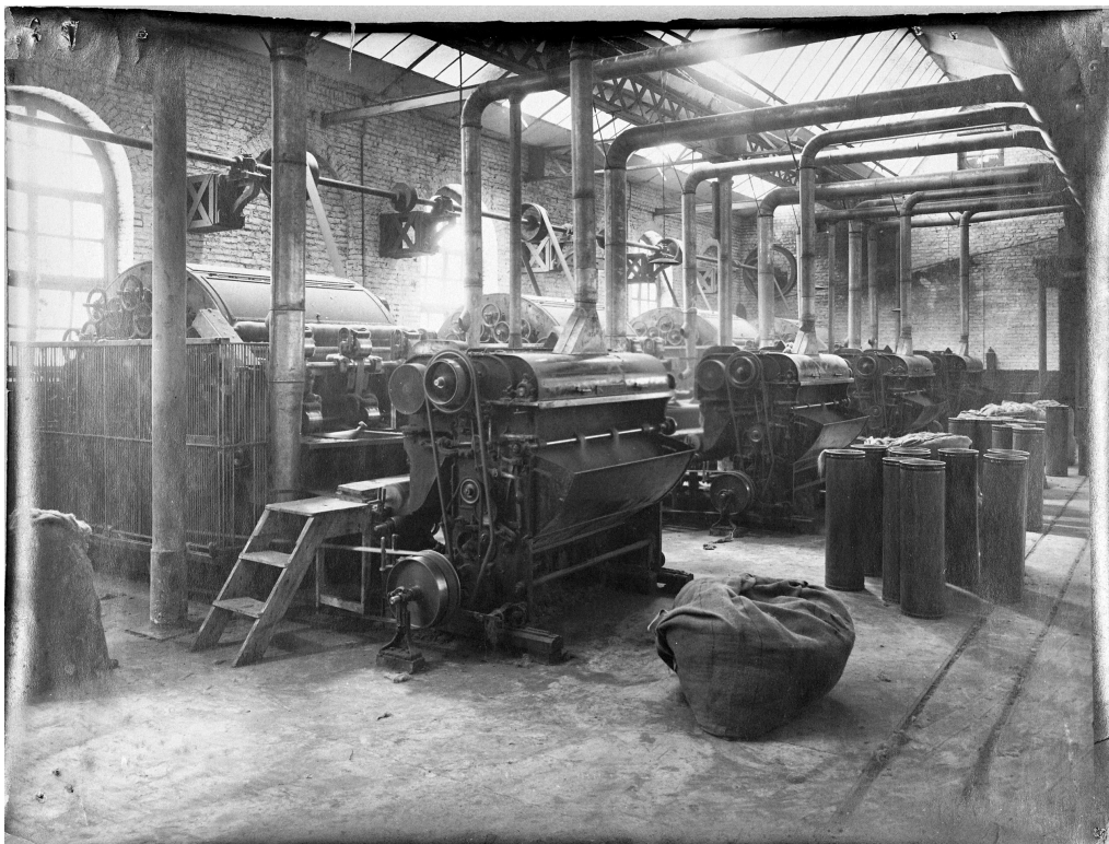
Ancienne filature. Cardeuses. Photographie, photographe inconnu, [circa 1900] (coll. part. Charvet).
